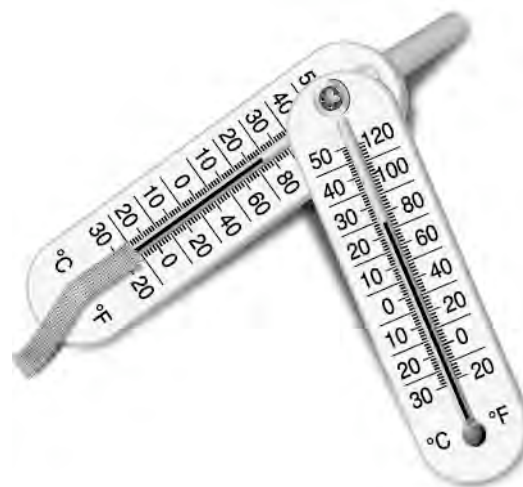
Figure 11-1. Assembled psychrometer.
