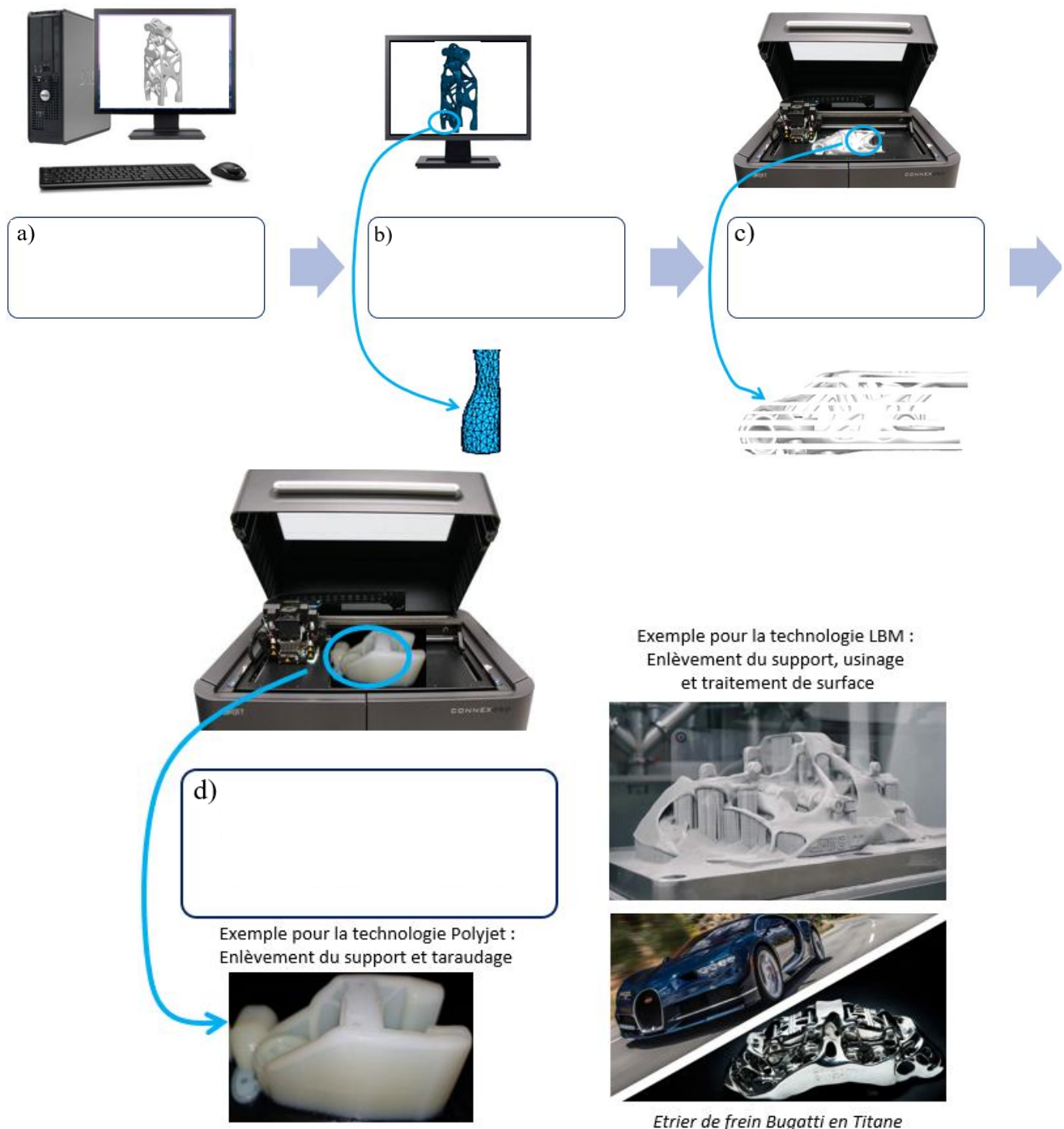
Figure 6 : Processus de la fabrication additive
