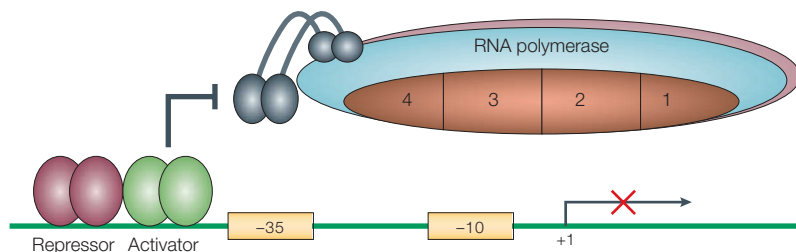
Figure 4 | Mechanisms of repression. a | Repression by steric hindrance. The repressor-binding site overlaps core promoter elements and blocks recognition of the promoter by the RNA polymerase holoenzyme. b | Repression by looping. Repressors bind to distal sites and interact by looping, repressing the intervening promoter. c | Repression by the modulation of an activator protein. The repressor binds to an activator and prevents the activator from functioning by blocking promoter recognition by the RNA polymerase holoenzyme.
